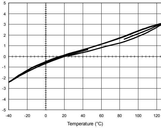
HAH1BV S/09 Gain Error (%)
