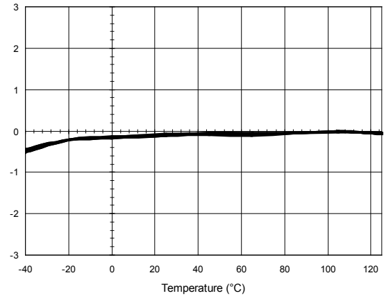
HAH1BV S/09 Electrical offset Error (A)
